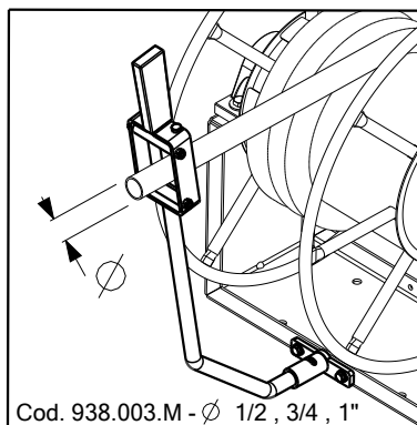
Guidatubo Manuale (Optional) Manual Hose-Guide (Optional)
